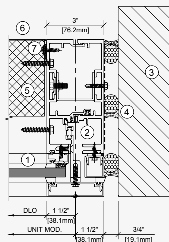
Detalle Jamba
