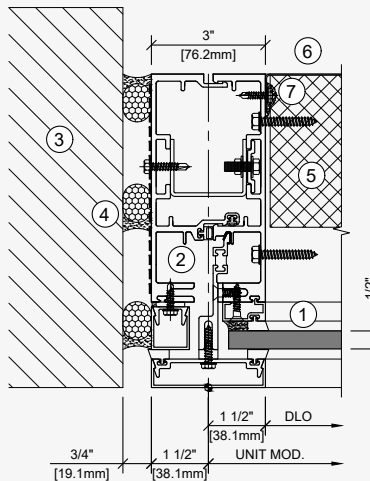
Detalle Jamba
