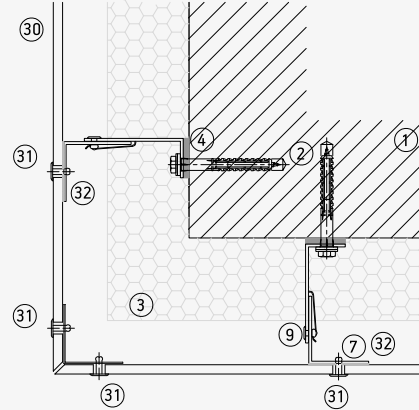
Junta vertical
