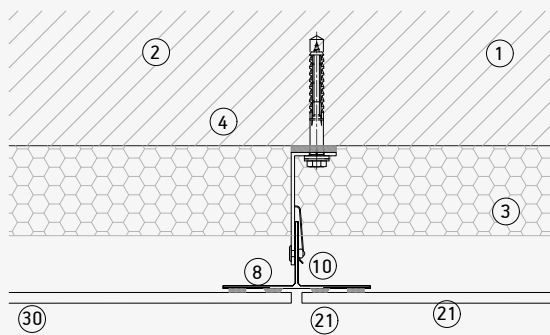
Junta vertical
