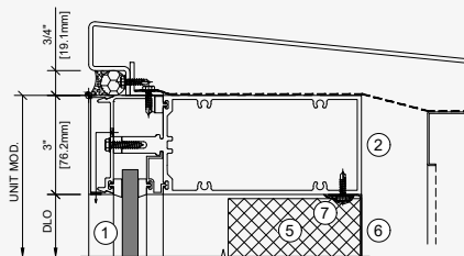
Remate Superior
